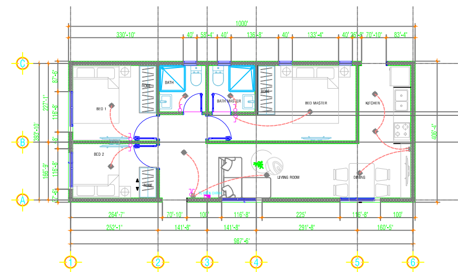
SWITCH LAYOUT
