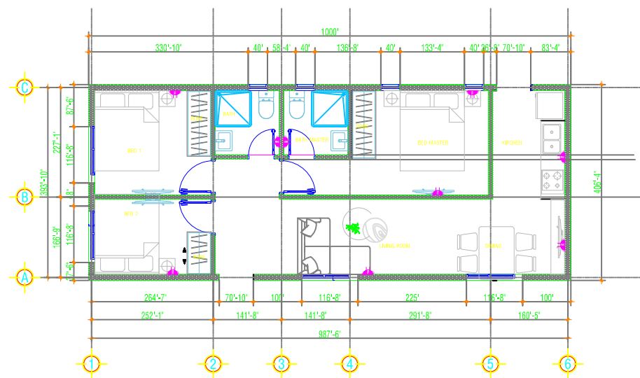
SOCKETS LAYOUT
