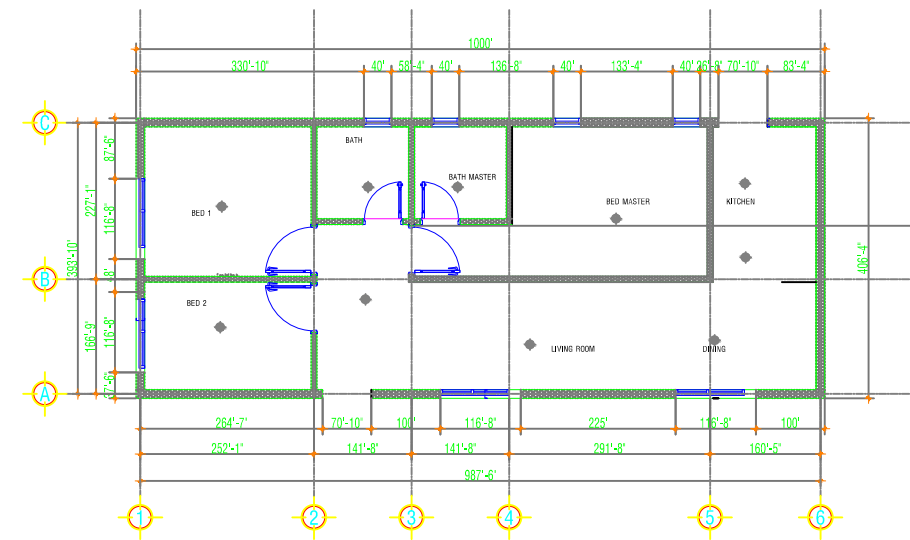
LIGHTING LAYOUT
